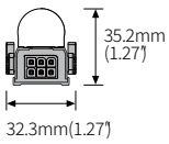
Without BRACKET
