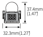
With BRACKET
