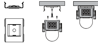
Standard mounting SSL-BRACKET
